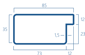
2D Kg/m 2.78
